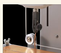
Copper foil peeling test with SC-8.
