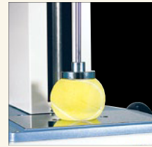
Ball compression test with S-40.
