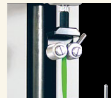
Rubber tube tension strength test with GP-15
