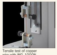
Tensile test of copper wire with WG-1000N
