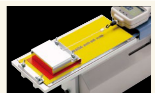
Paper coefficient of friction test with COF2-10N
