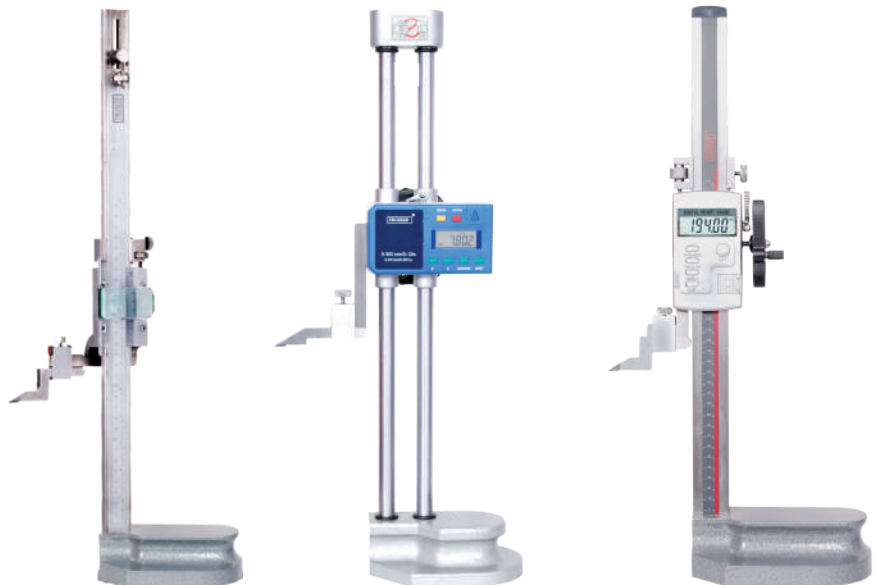
Height Gauges
