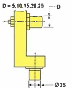
Gooseneck anvil for pipe 5 to 25 mm ID with 5 mm step
