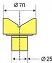
Testing table of Ø 70 mm with V groove for jobs Ø 10 to 80 mm
