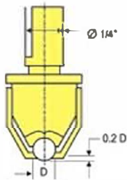
Steel Ball Indenter Dia. (1/16", 1/4", 3/8", 1/2" 2.5mm, 5mm)
