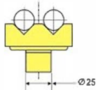
Cylindron anvil for testing big job from Ø50 mm to Ø150 mm
