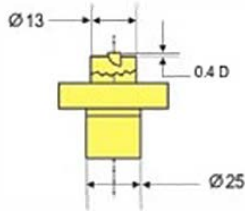
Diamond spot anvil
