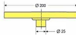
Testing Table Ø 200 mm Hardened & Ground
