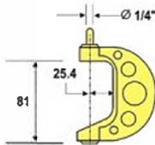
Gooseneck adaptor No.3
