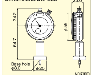
Dimensions:DM-283
